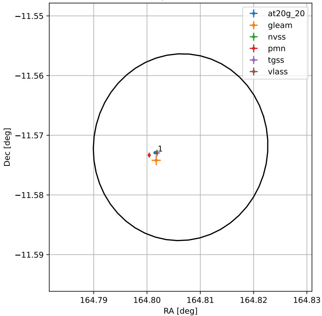
4FGL J1059.2-1134
