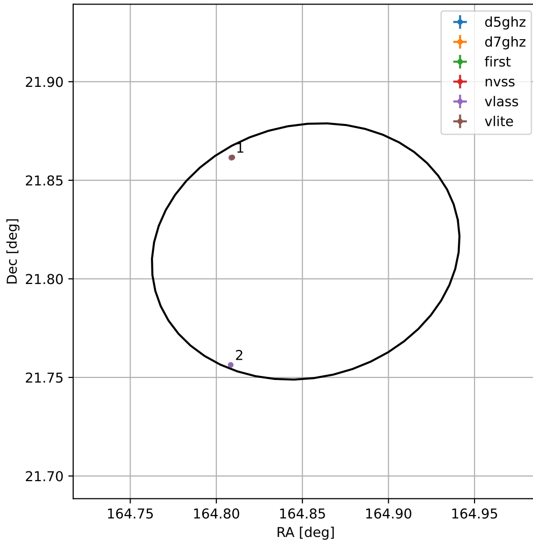
4FGL J1059.4+2148
