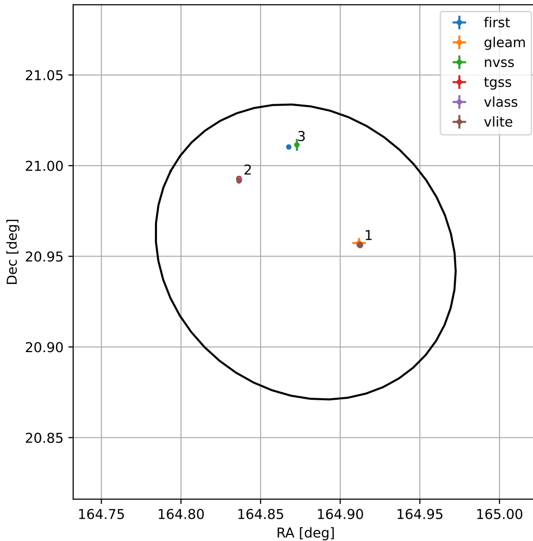
4FGL J1059.5+2057
