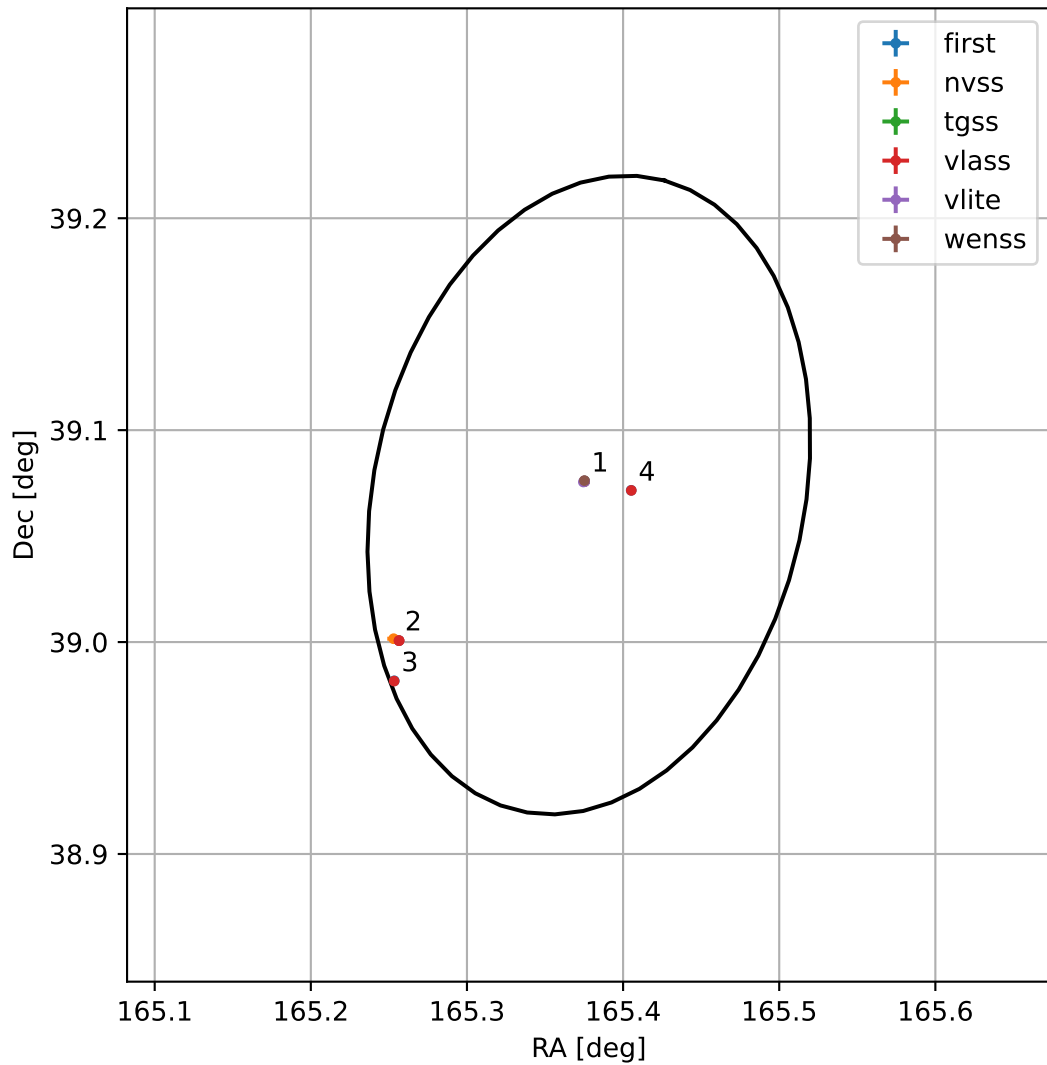
4FGL J1101.5+3904
