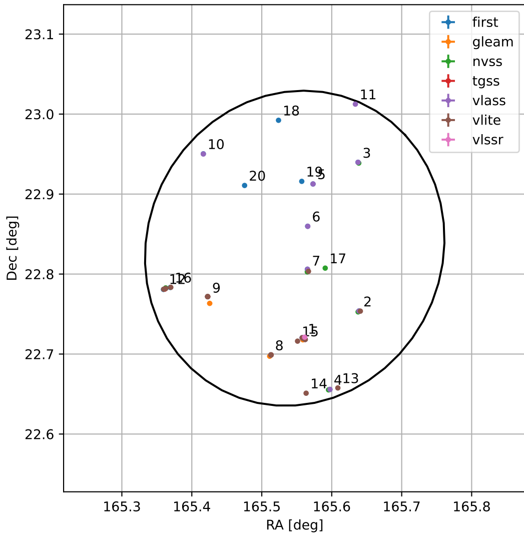
4FGL J1102.1+2249
