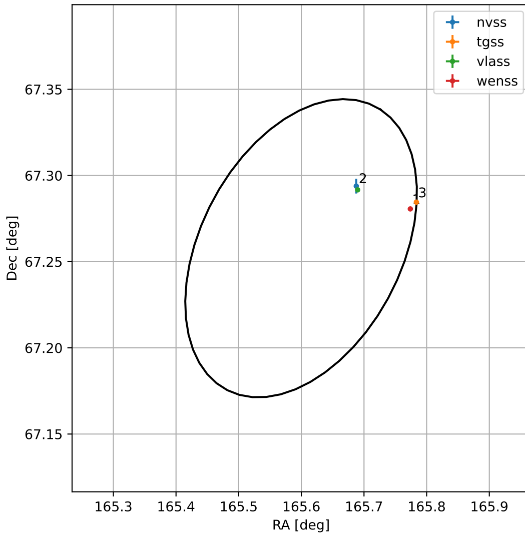
4FGL J1102.3+6715
