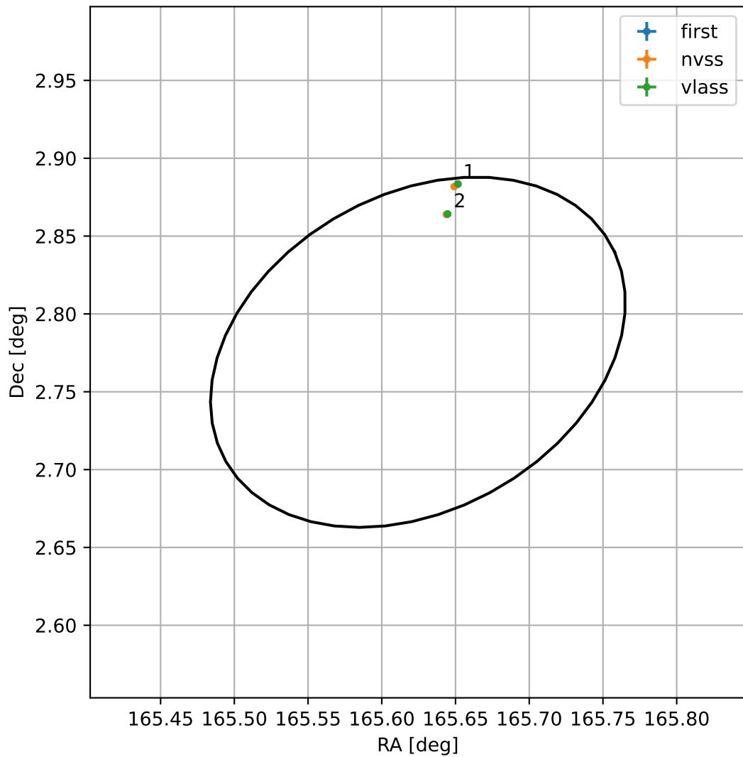
4FGL J1102.4+0246
