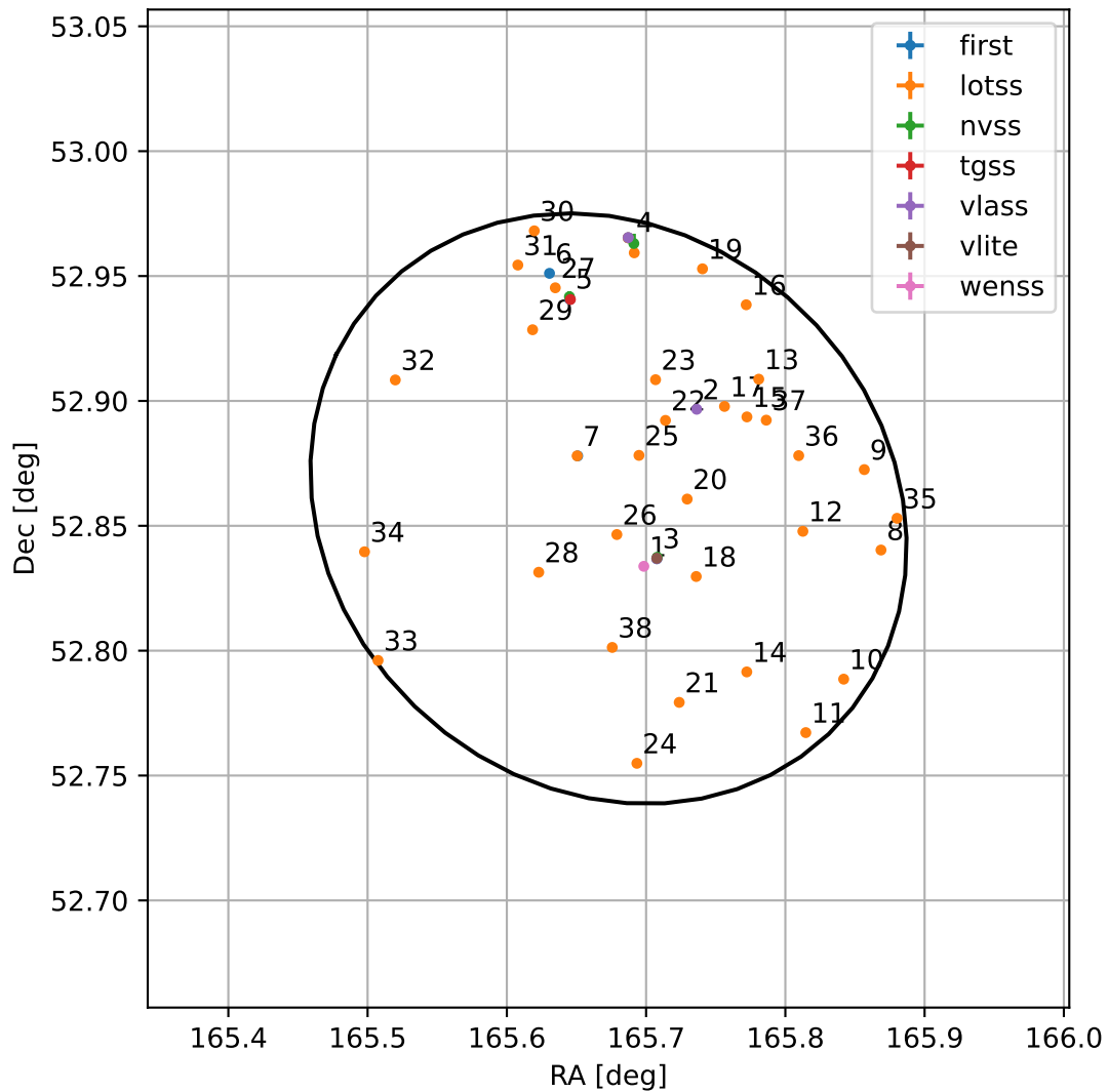
4FGL J1102.6+5251
