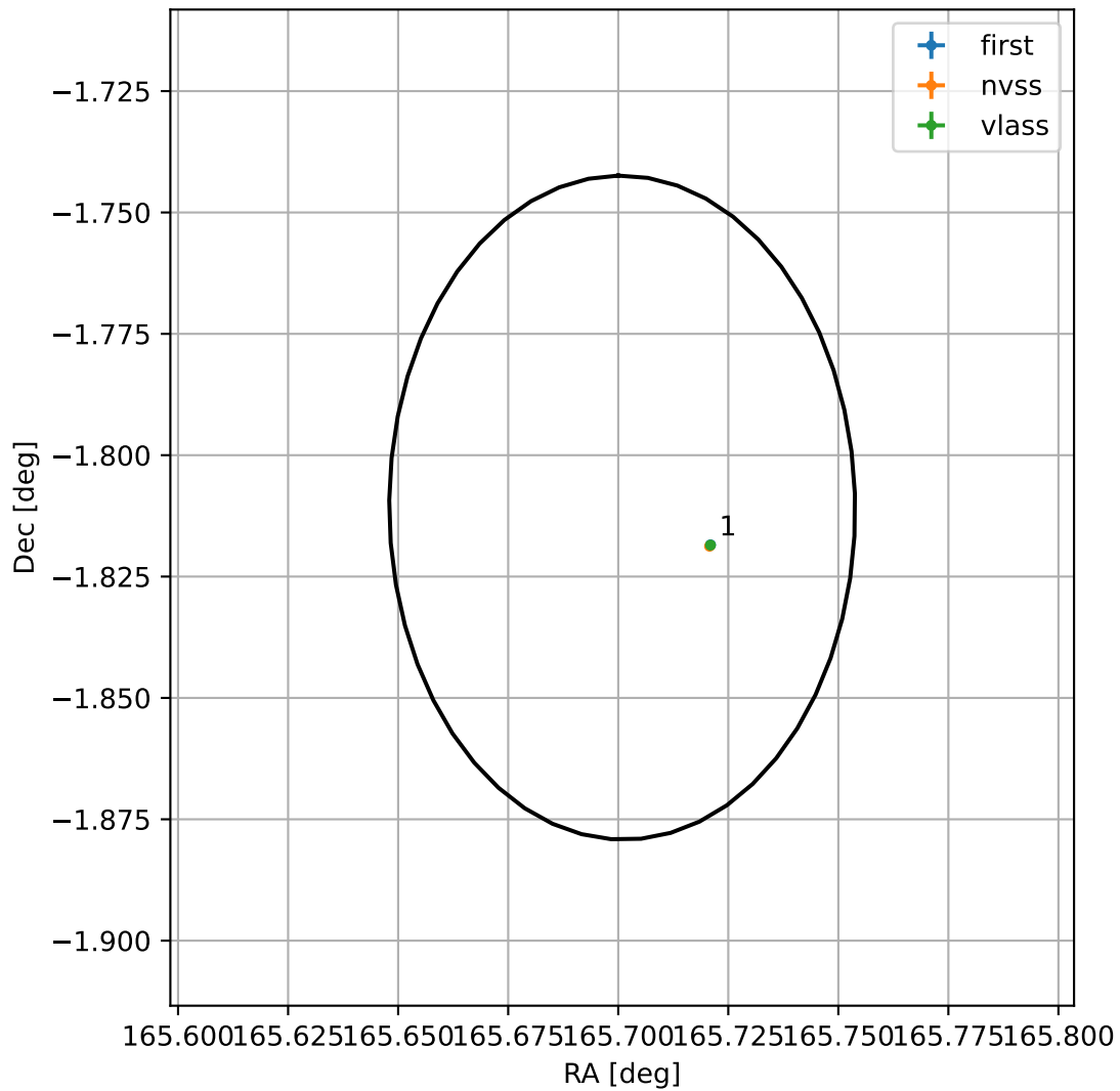
4FGL J1102.8-0148
