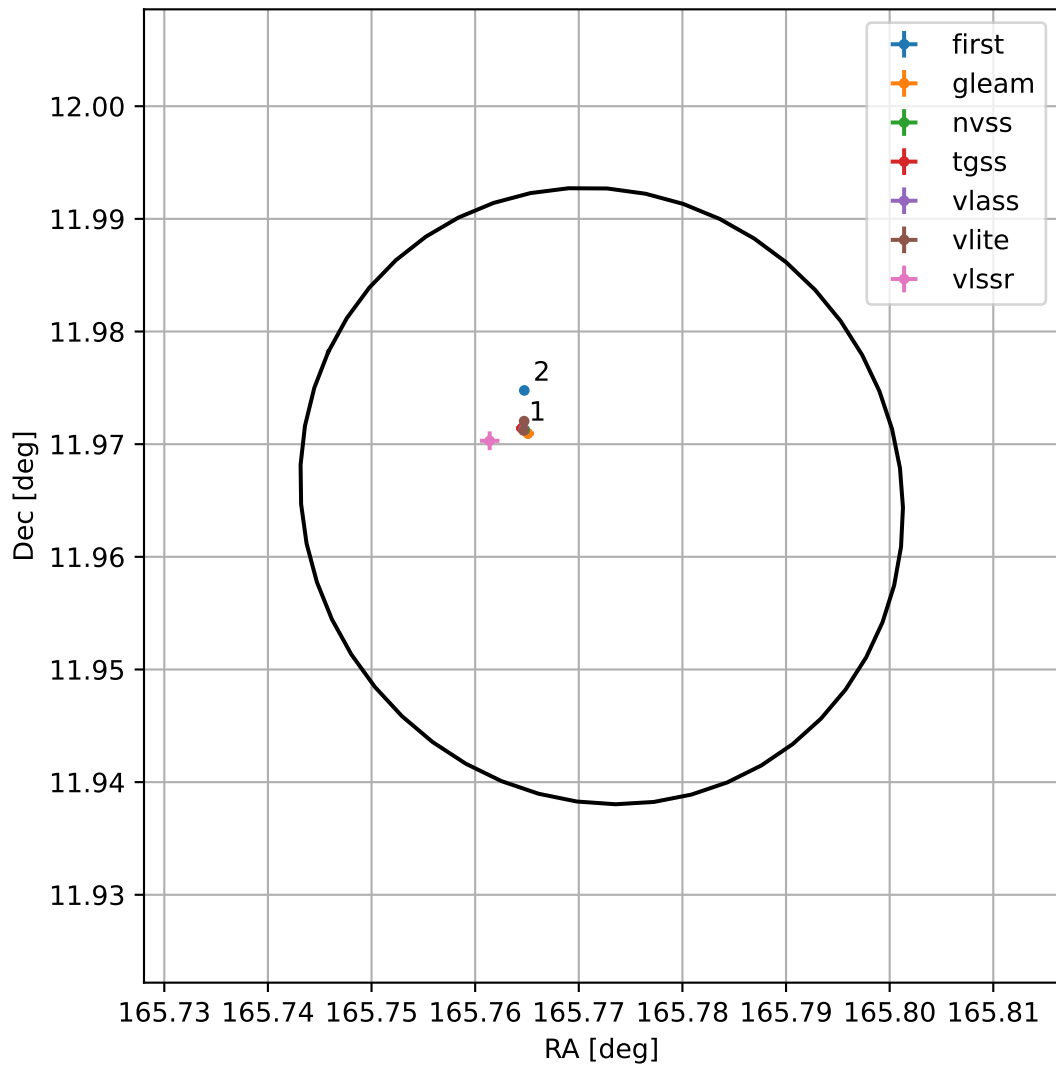
4FGL J1103.0+1157
