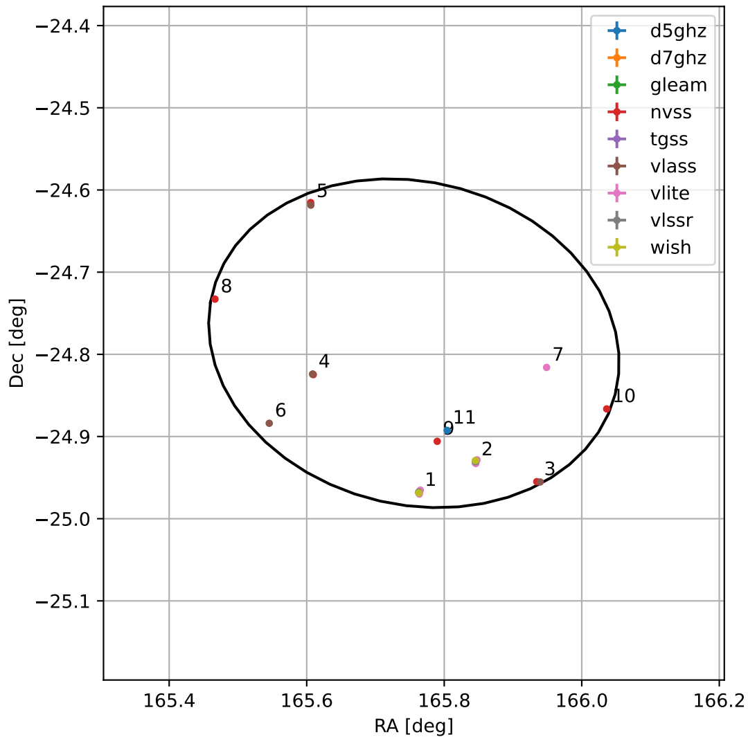
4FGL J1103.0-2447
