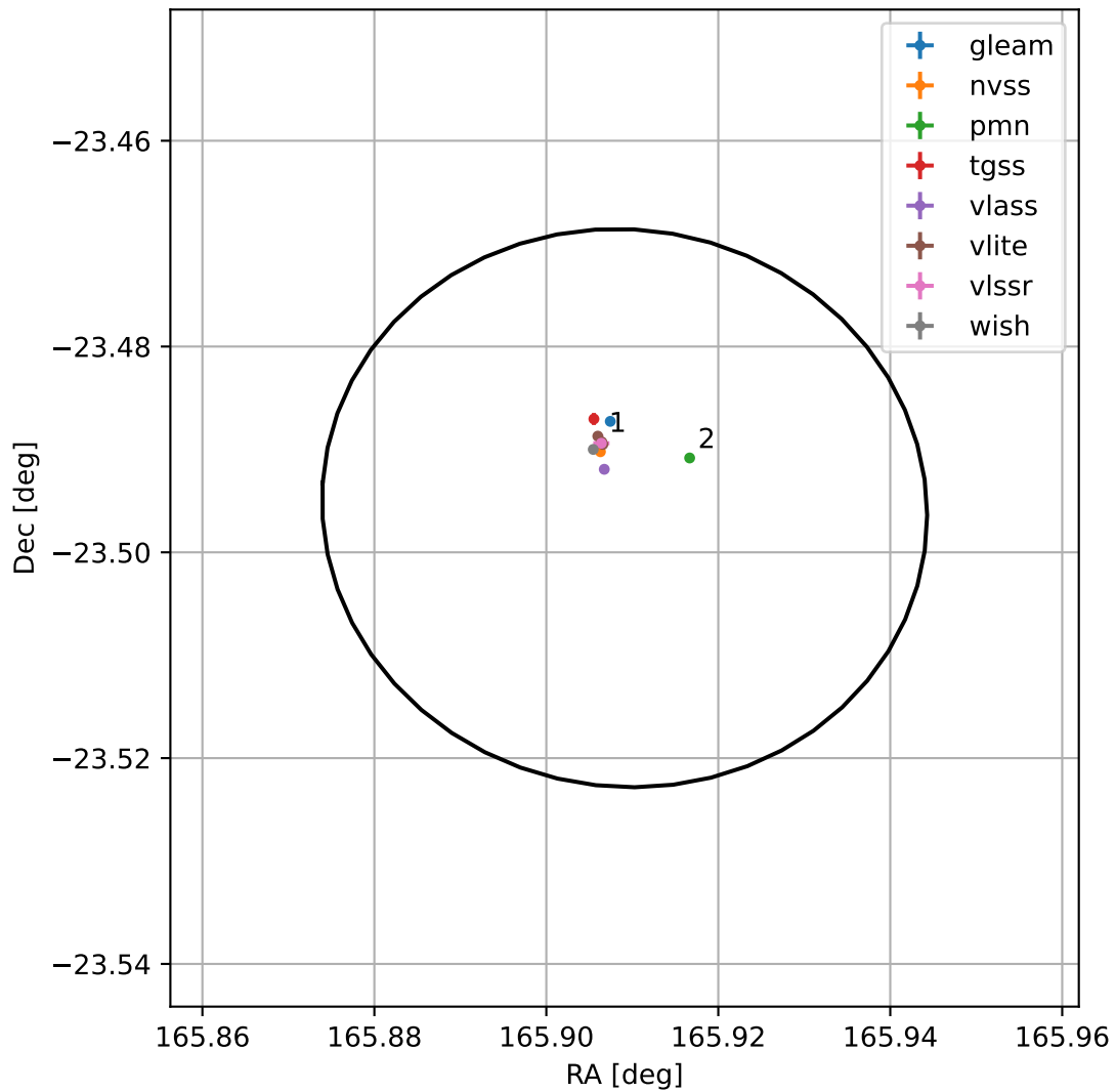
4FGL J1103.6-2329
