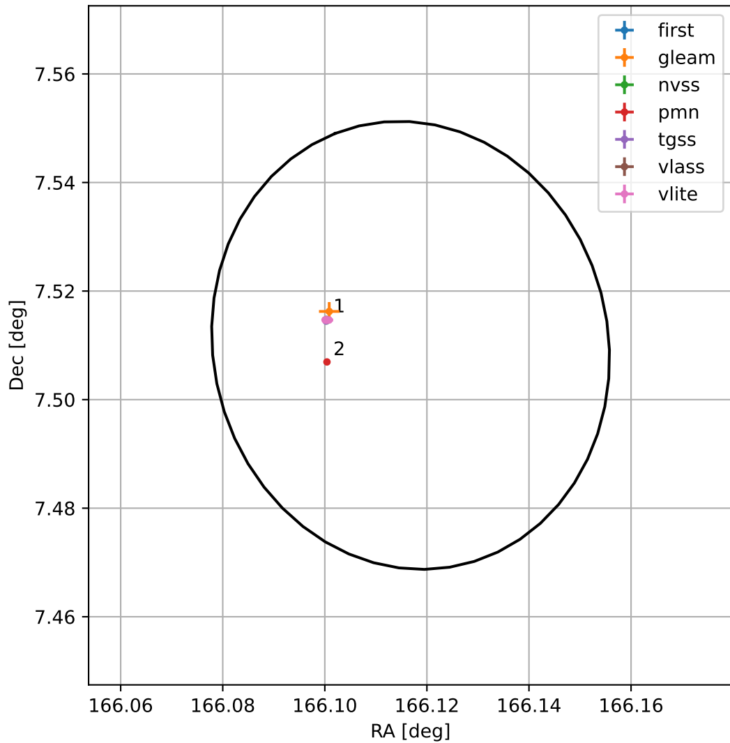
4FGL J1104.4+0730
