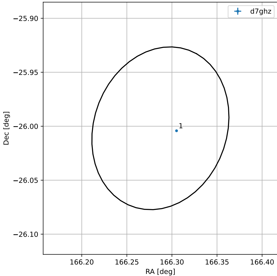
4FGL J1105.1-2600
