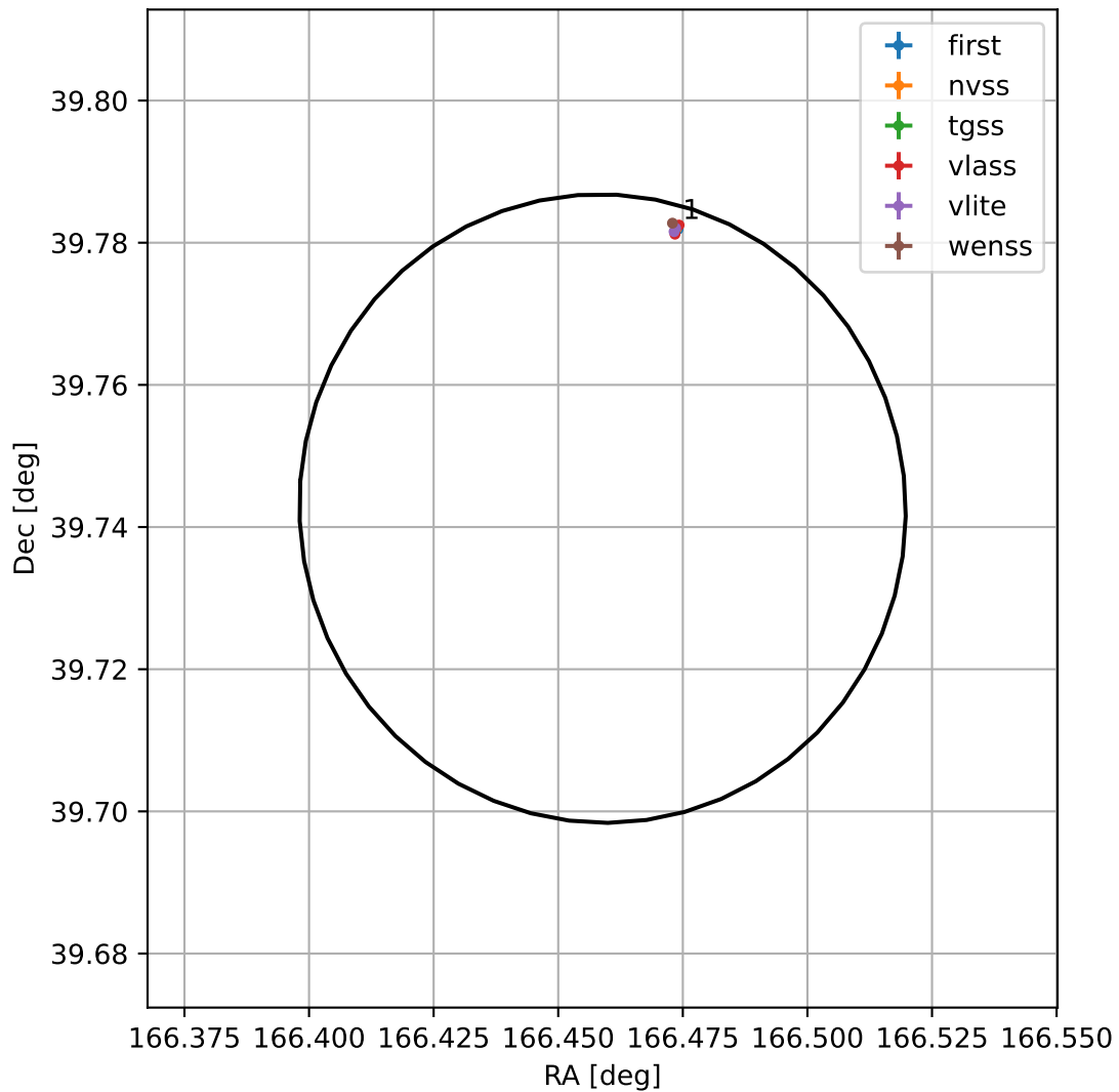
4FGL J1105.8+3944
