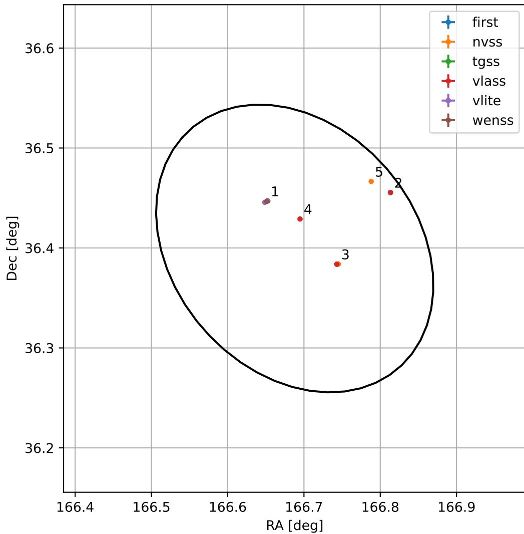
4FGL J1106.7+3623
