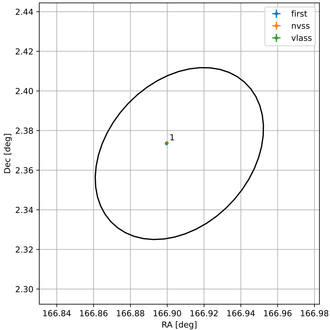
4FGL J1107.6+0222
