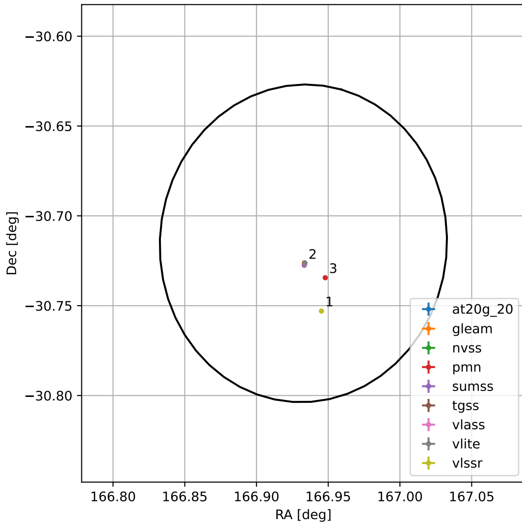
4FGL J1107.7-3042
