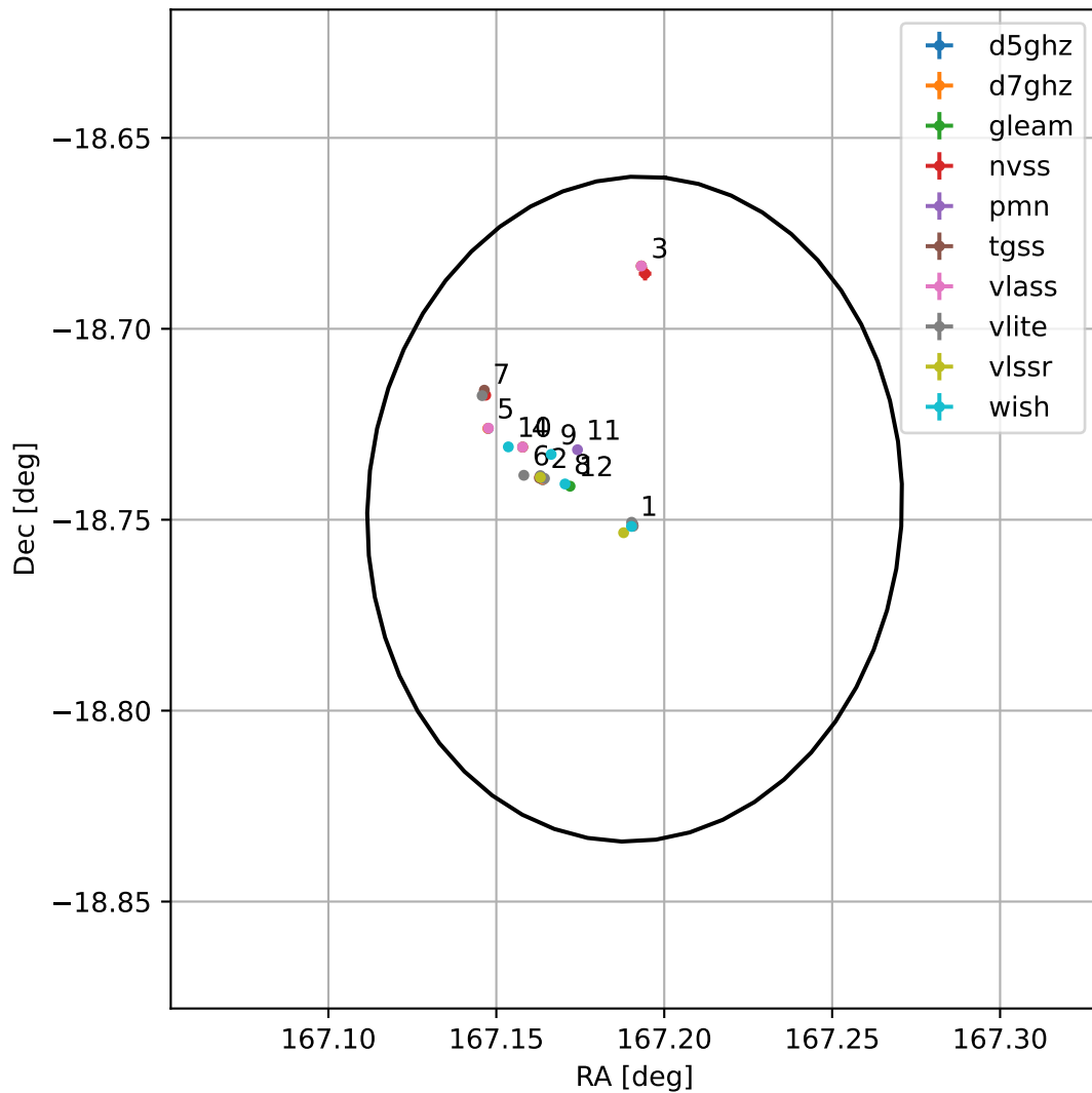
4FGL J1108.7-1844
