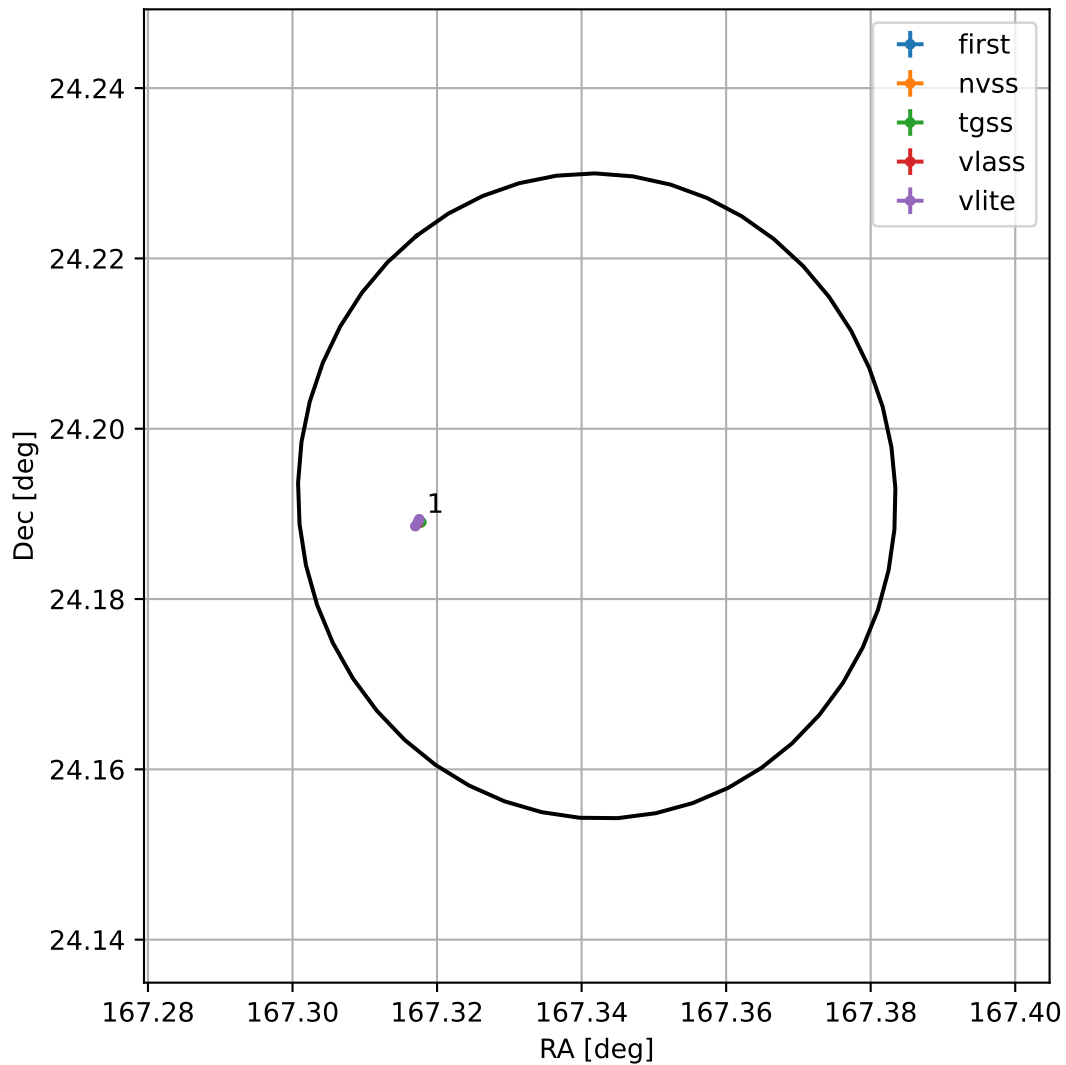
4FGL J1109.3+2411
