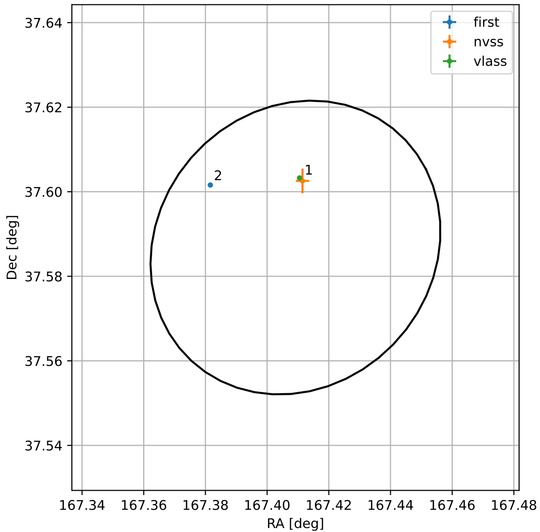
4FGL J1109.6+3735
