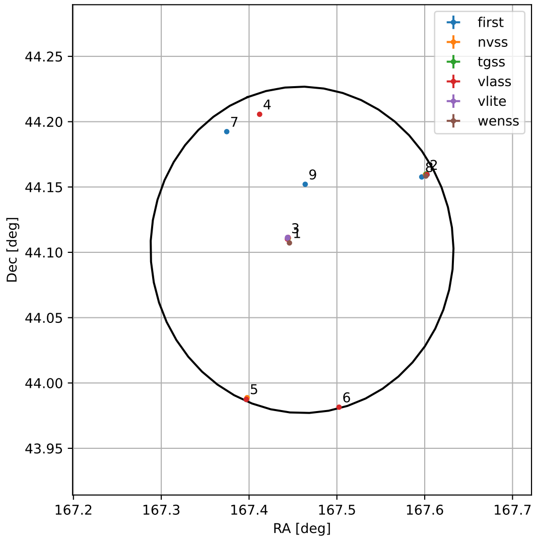
4FGL J1109.8+4406
