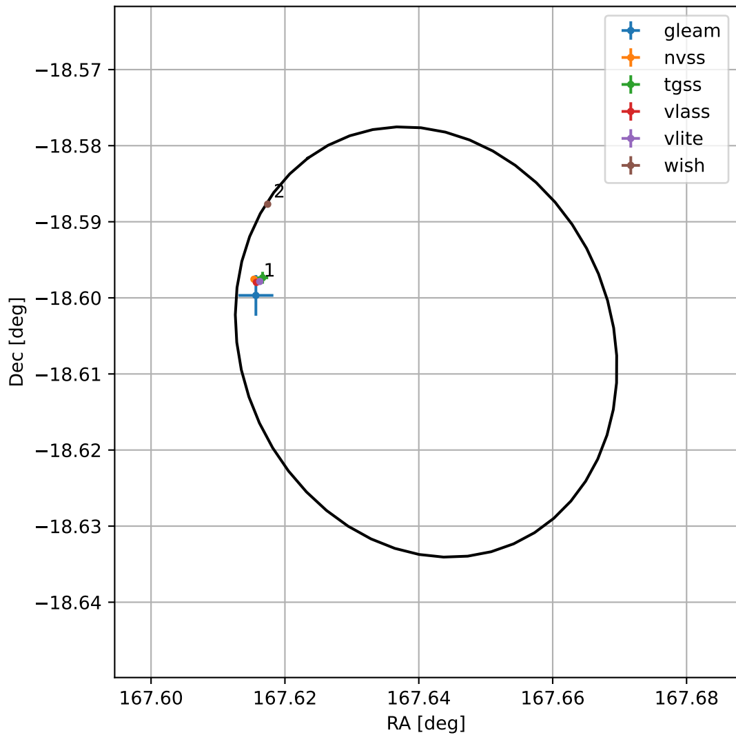
4FGL J1110.5-1836
