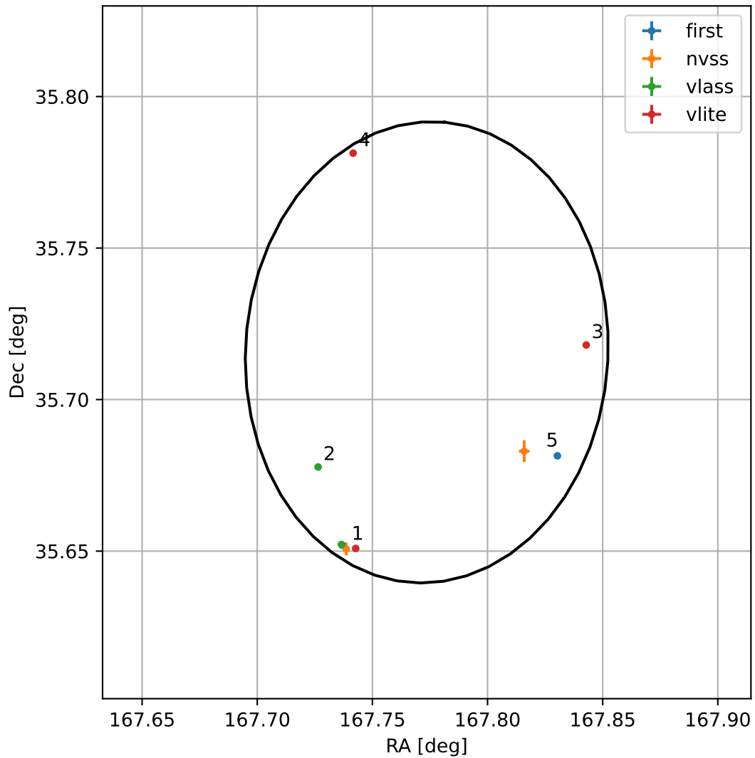
4FGL J1111.0+3542
