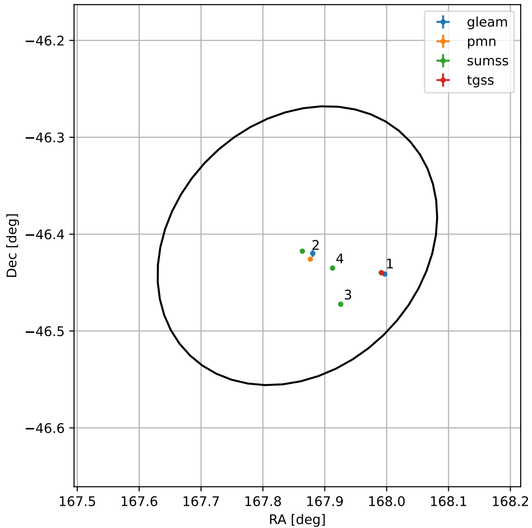
4FGL J1111.4-4624
