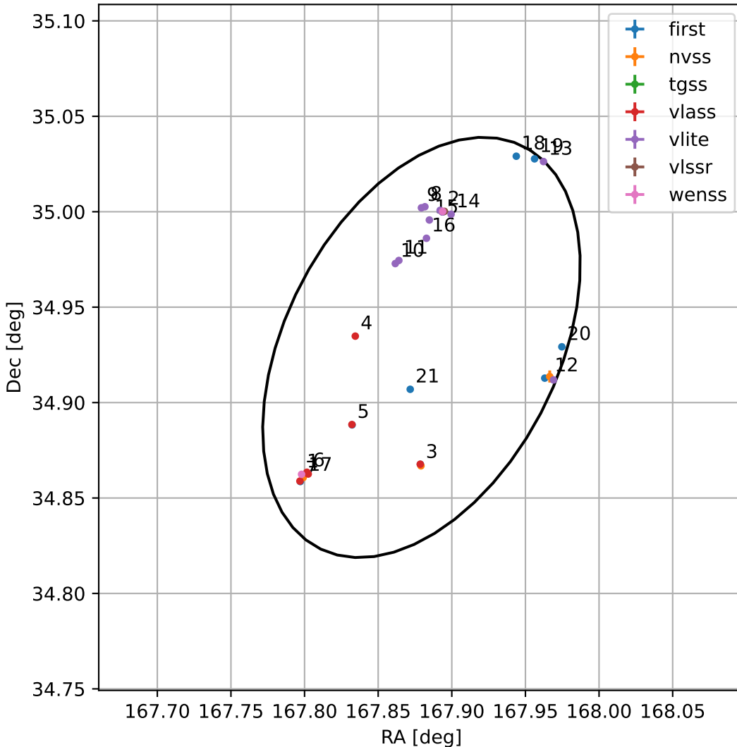
4FGL J1111.5+3455
