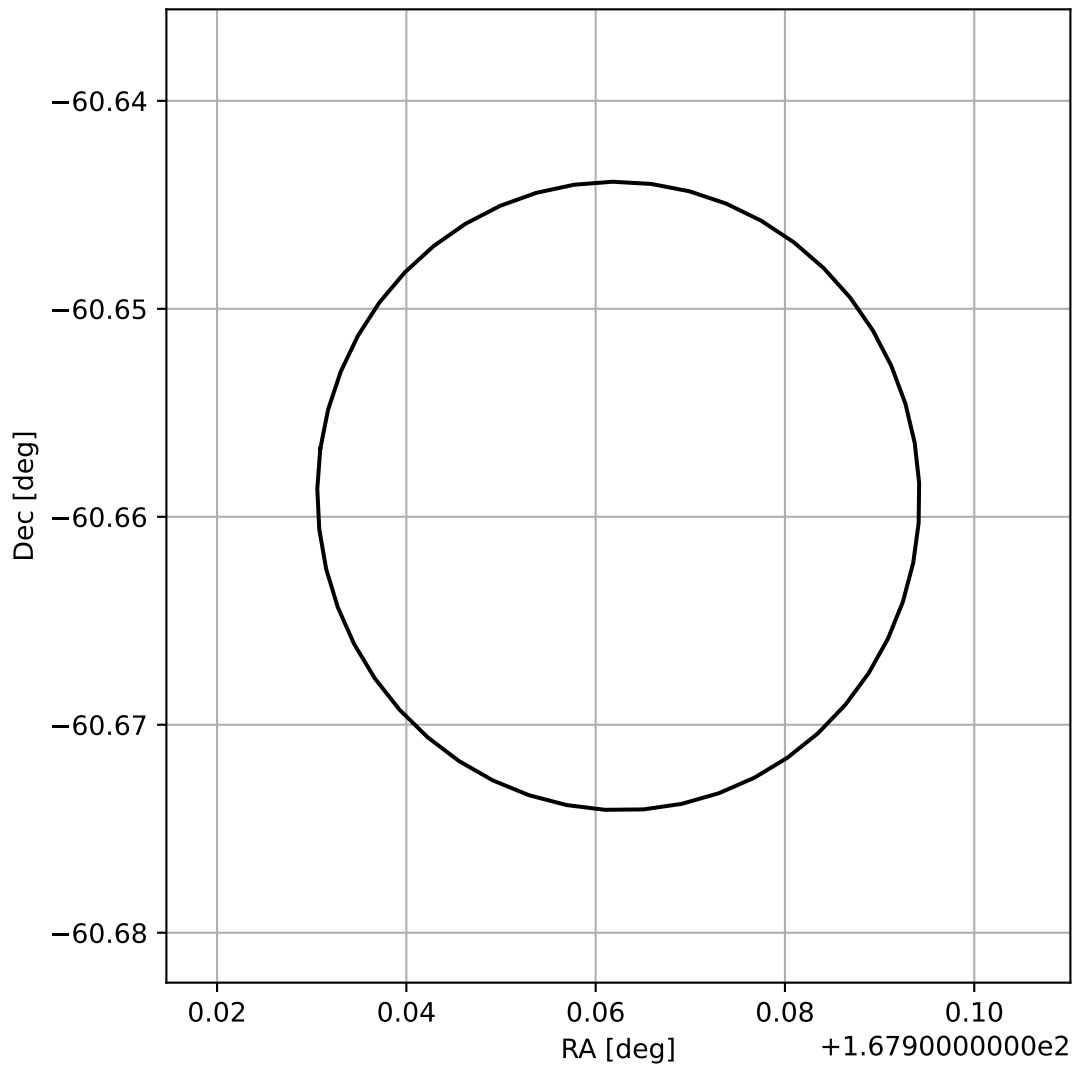
4FGL J1111.8-6039
