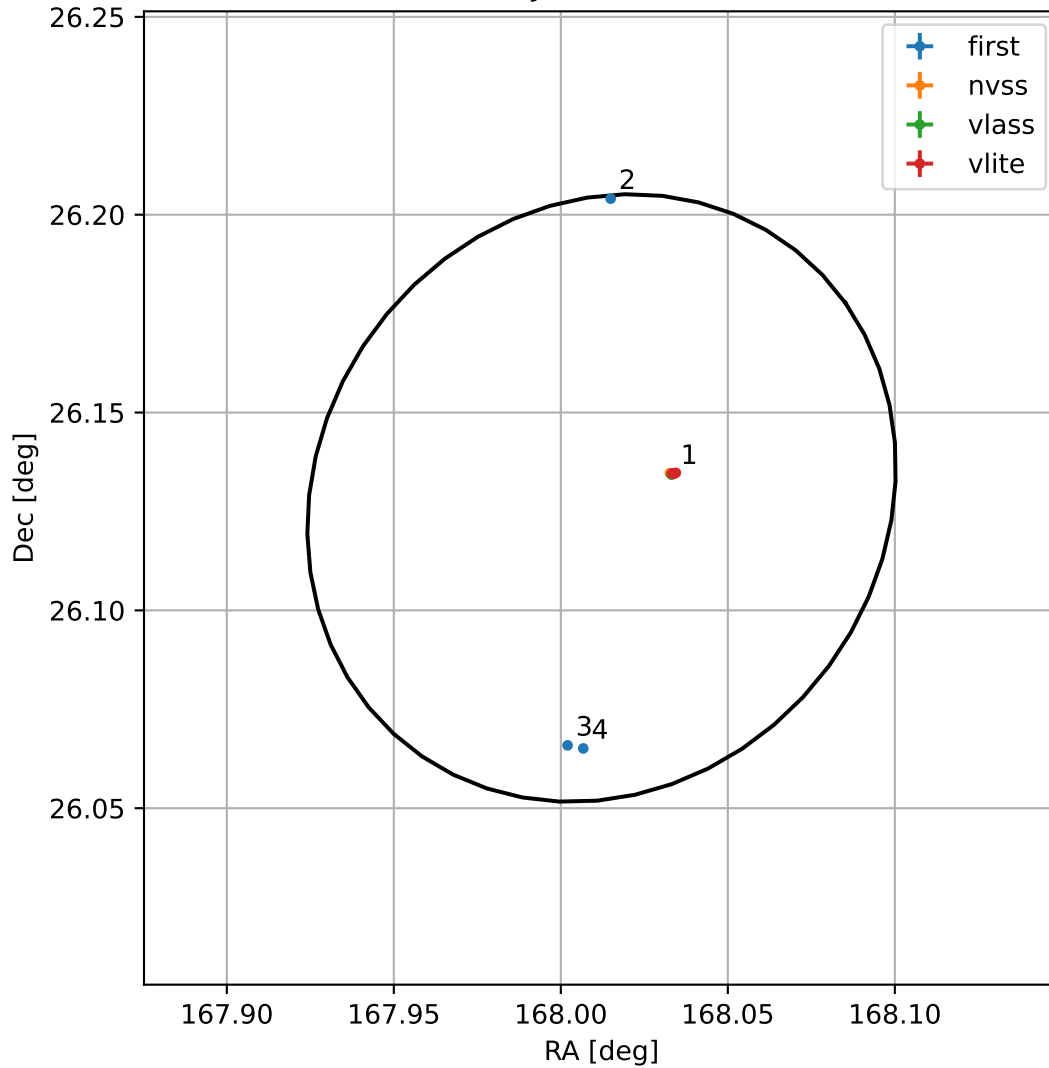
4FGL J1112.0+2607
