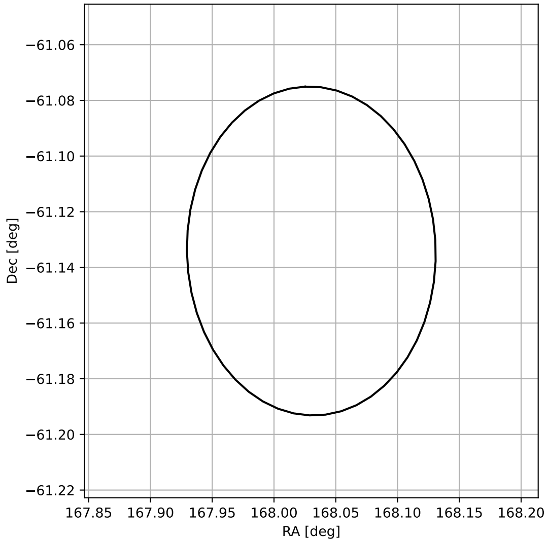
4FGL J1112.1-6108
