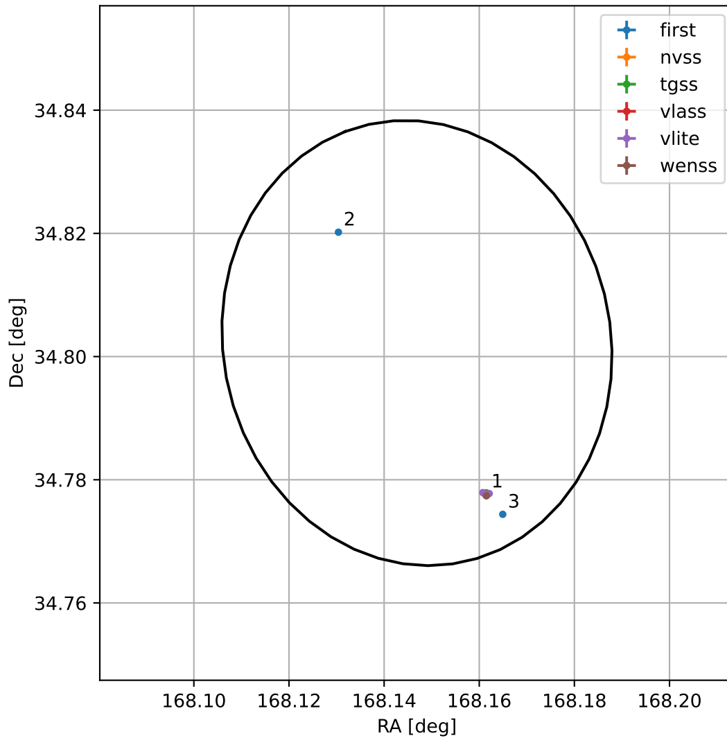
4FGL J1112.5+3448
