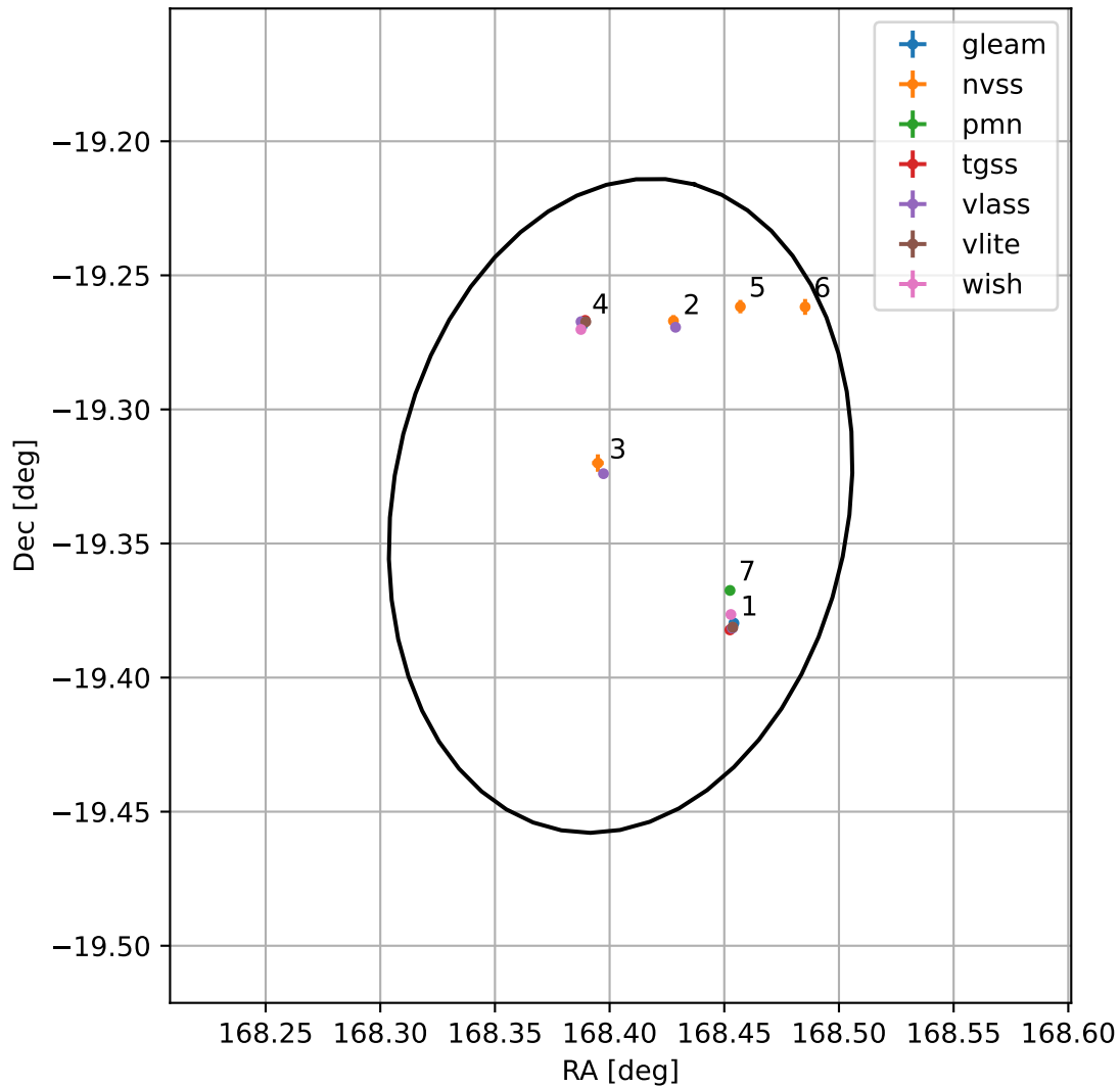
4FGL J1113.6-1920
