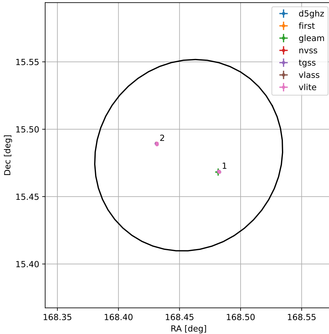
4FGL J1113.8+1528
