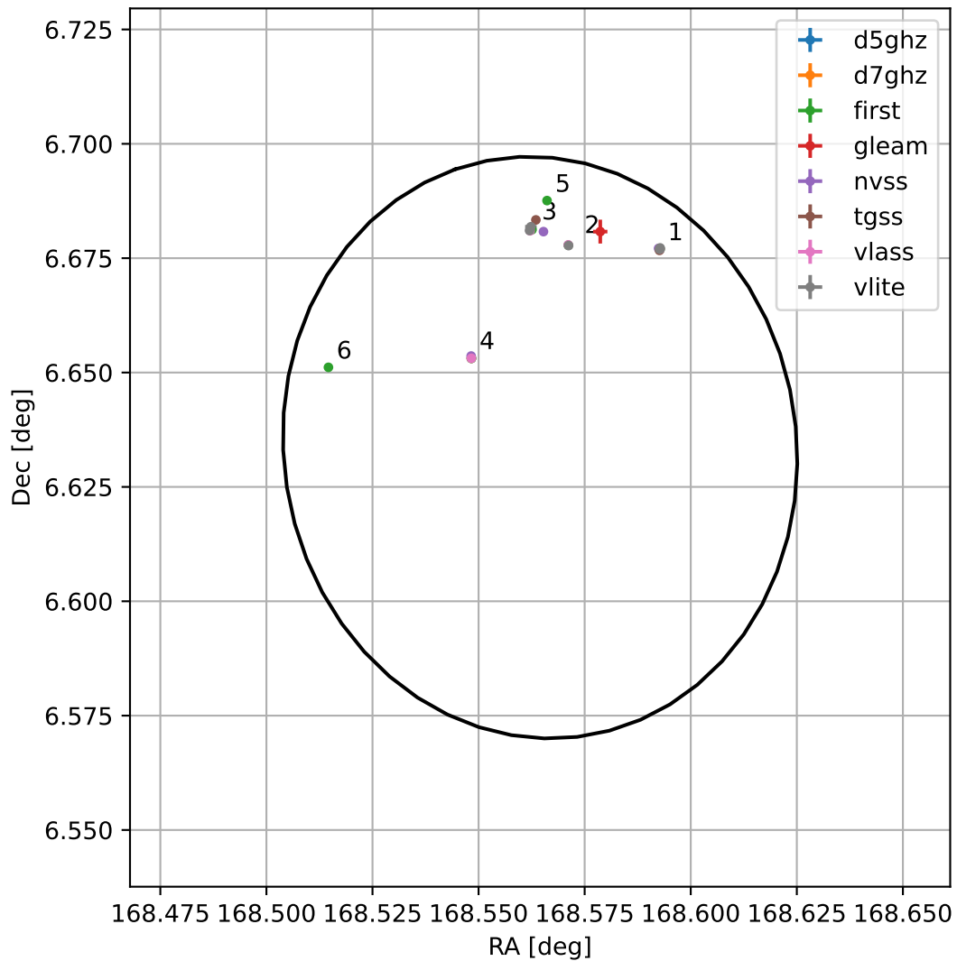
4FGL J1114.2+0638
