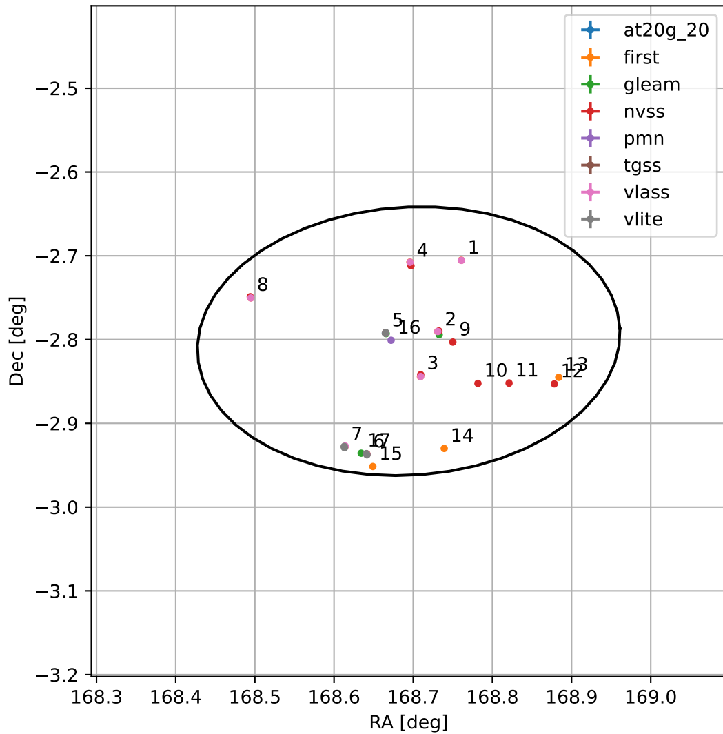
4FGL J1114.7-0248
