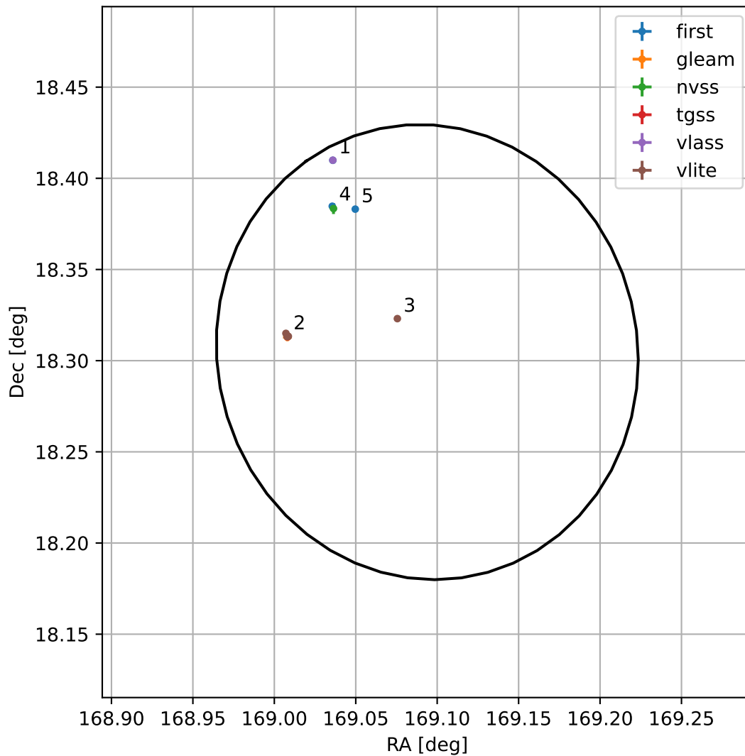
4FGL J1116.3+1818
