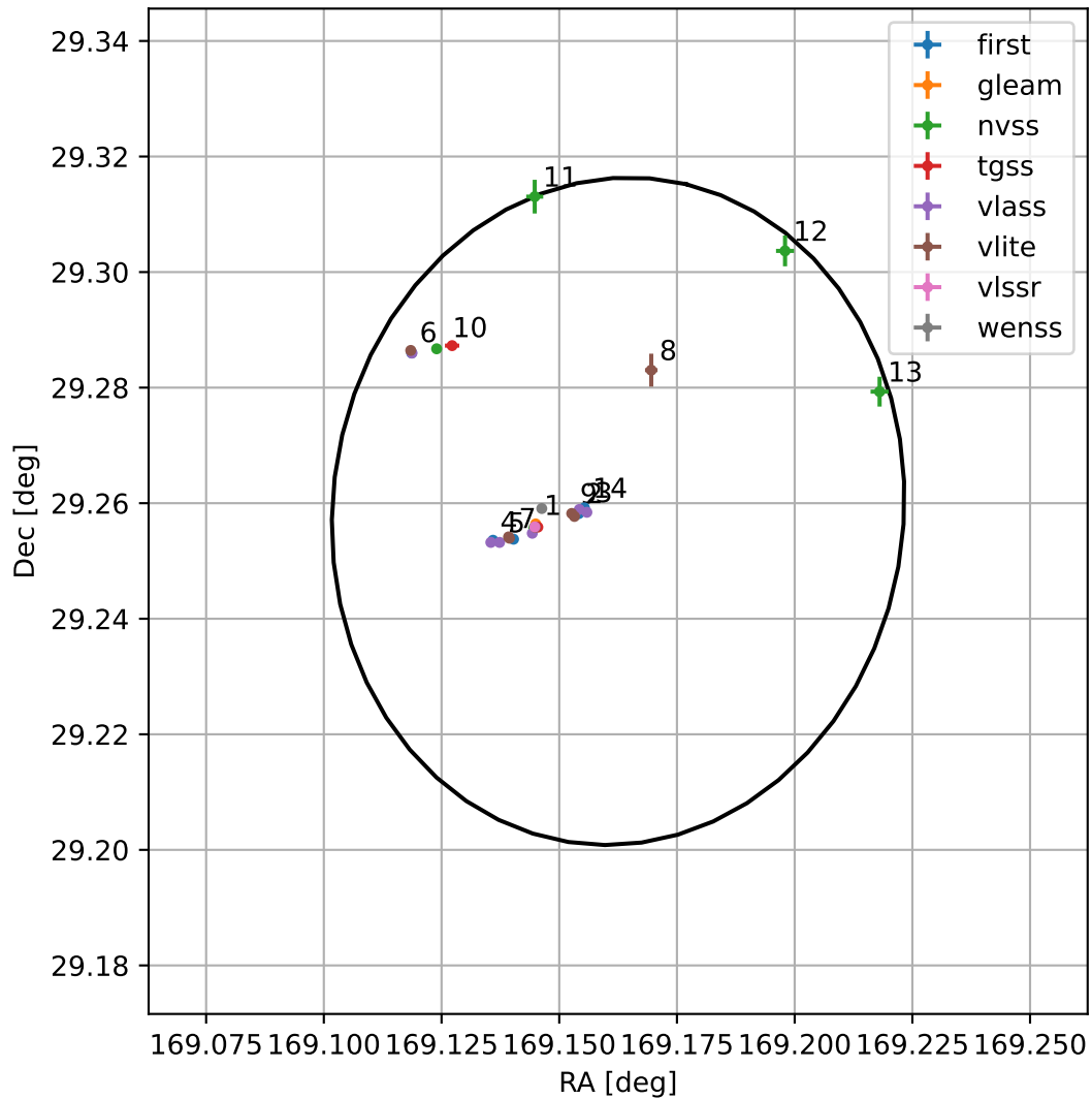
4FGL J1116.6+2915
