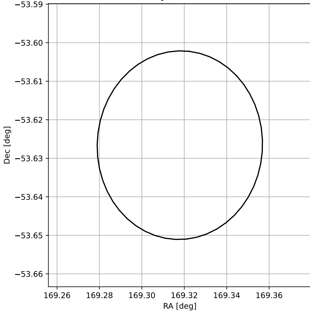
4FGL J1117.2-5337
