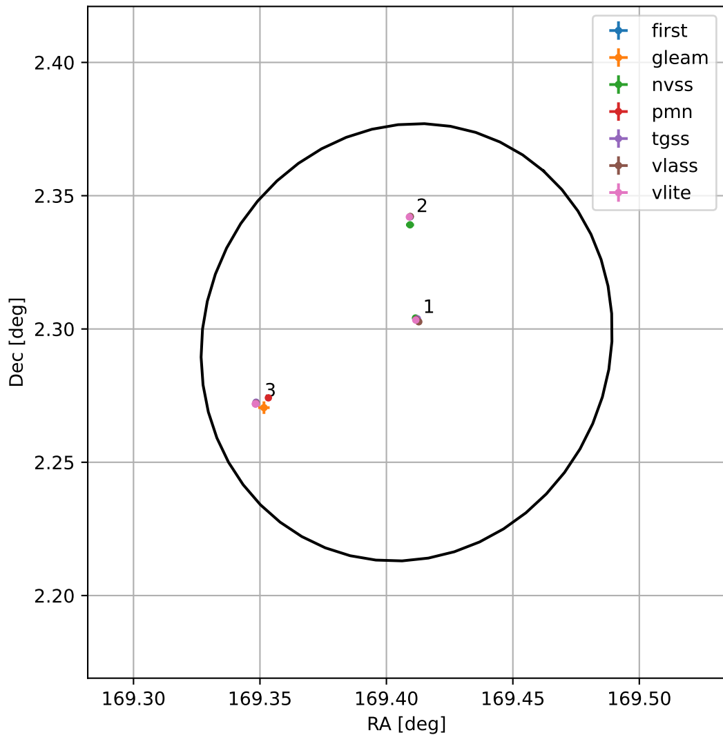
4FGL J1117.6+0217
