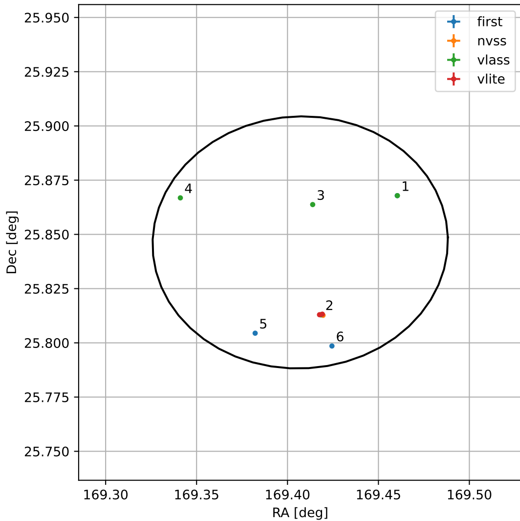
4FGL J1117.6+2550
