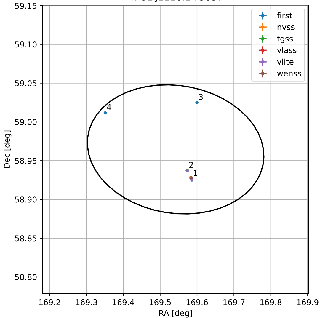
4FGL J1118.1+5857
