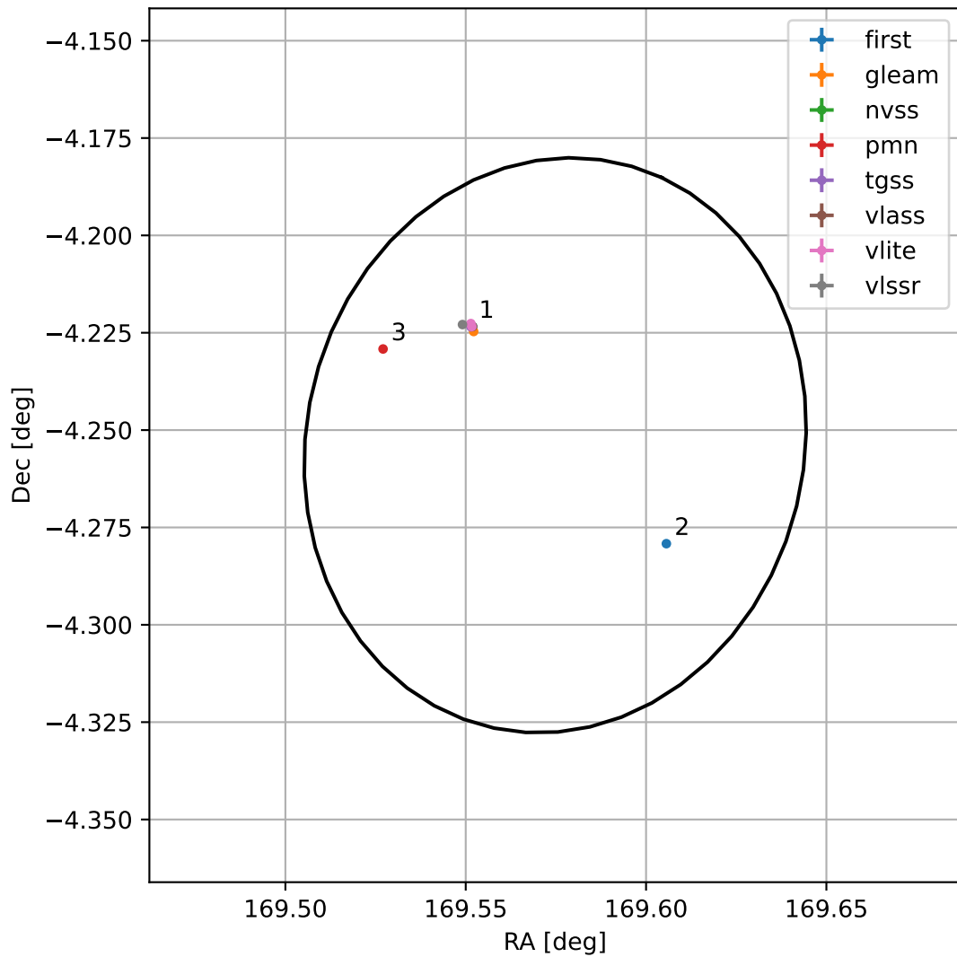
4FGL J1118.2-0415
