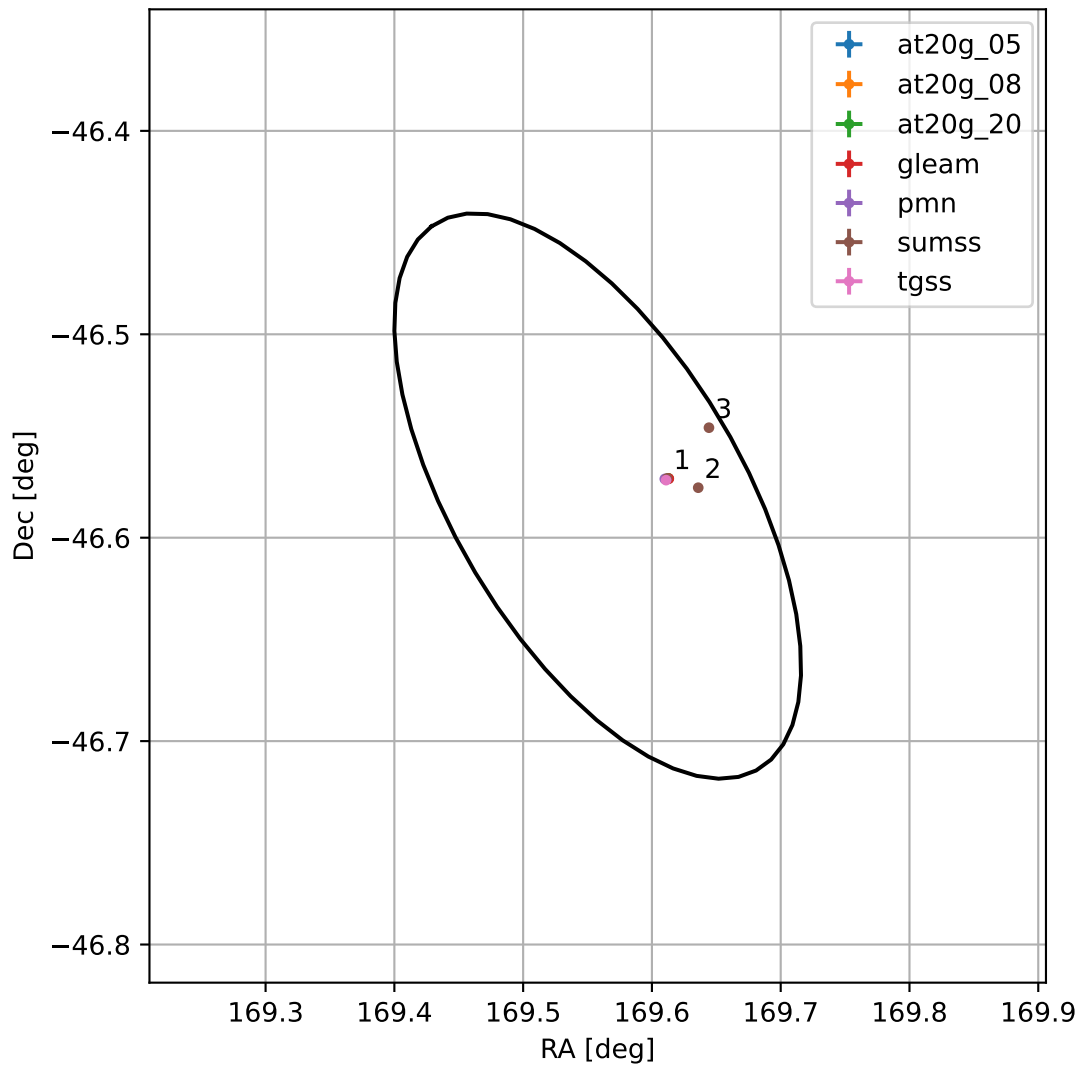
4FGL J1118.2-4634
