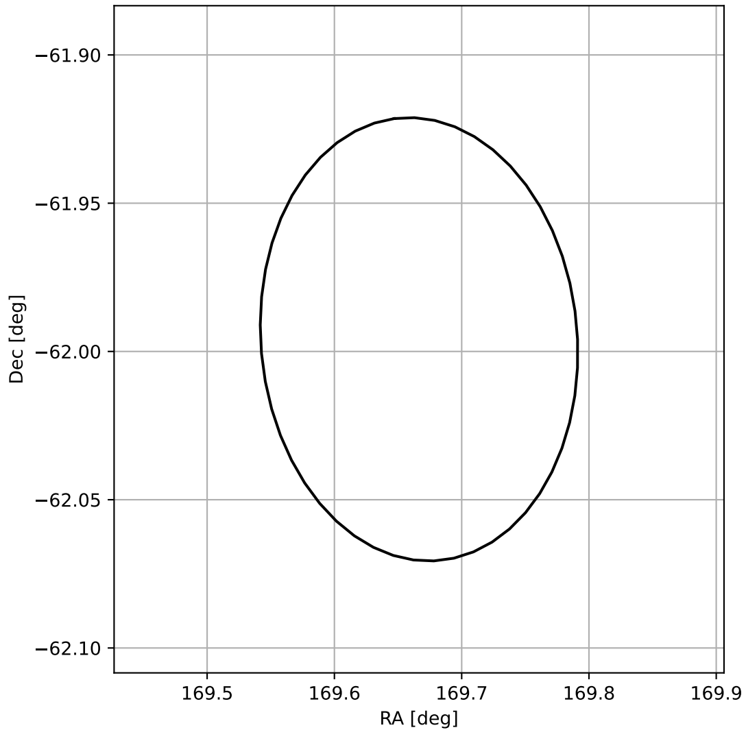
4FGL J1118.6-6159
