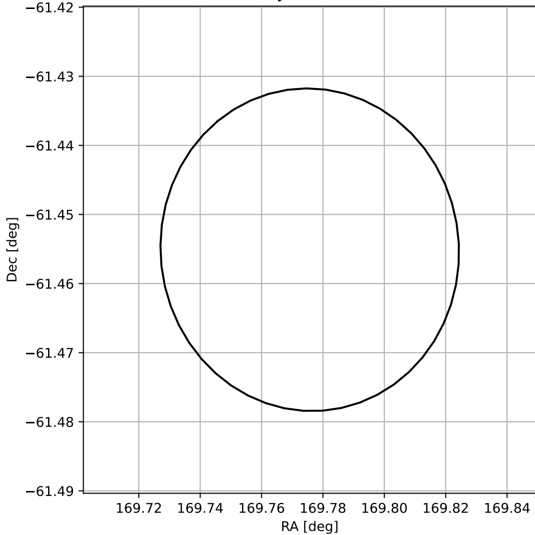
4FGL J1119.1-6127
