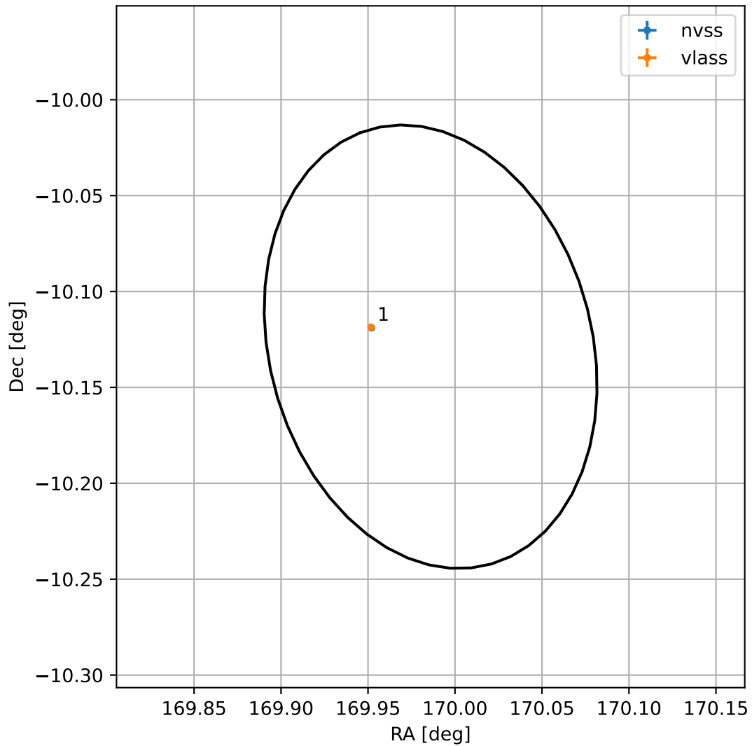
4FGL J1119.9-1007
