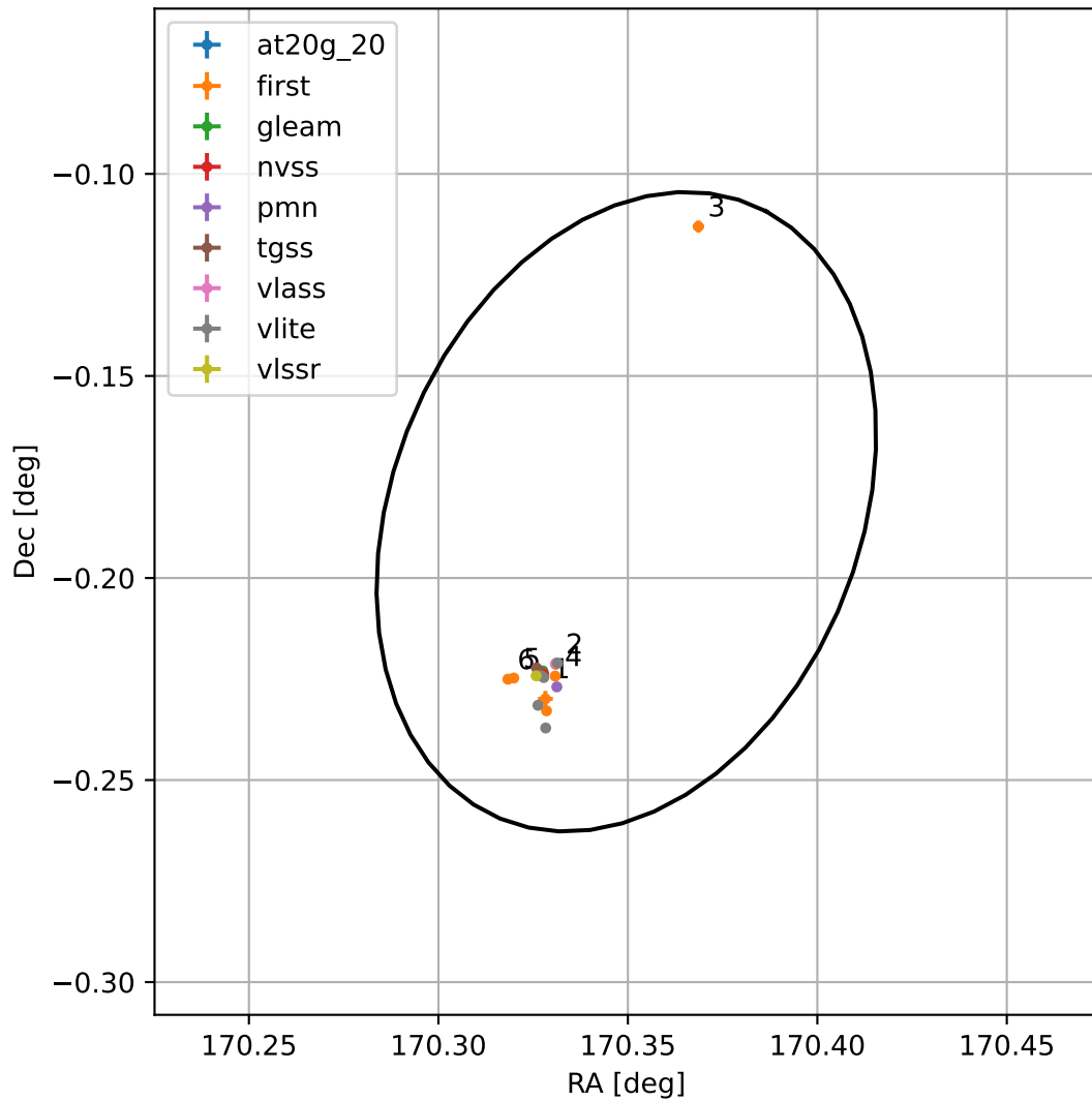
4FGL J1121.3-0011
