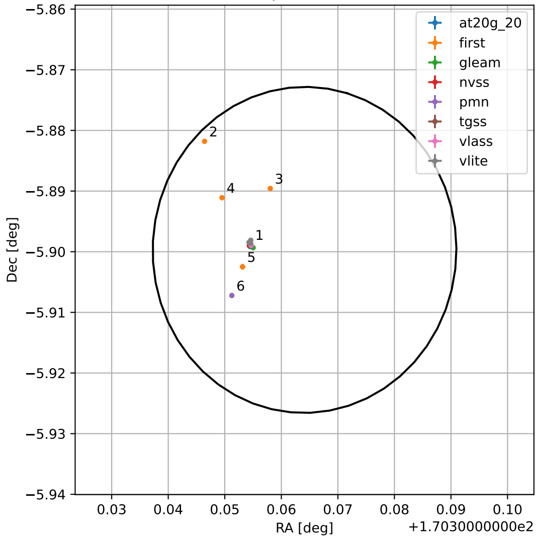
4FGL J1121.4-0553
