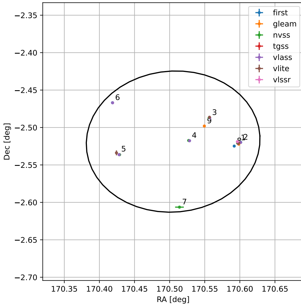
4FGL J1122.0-0231
