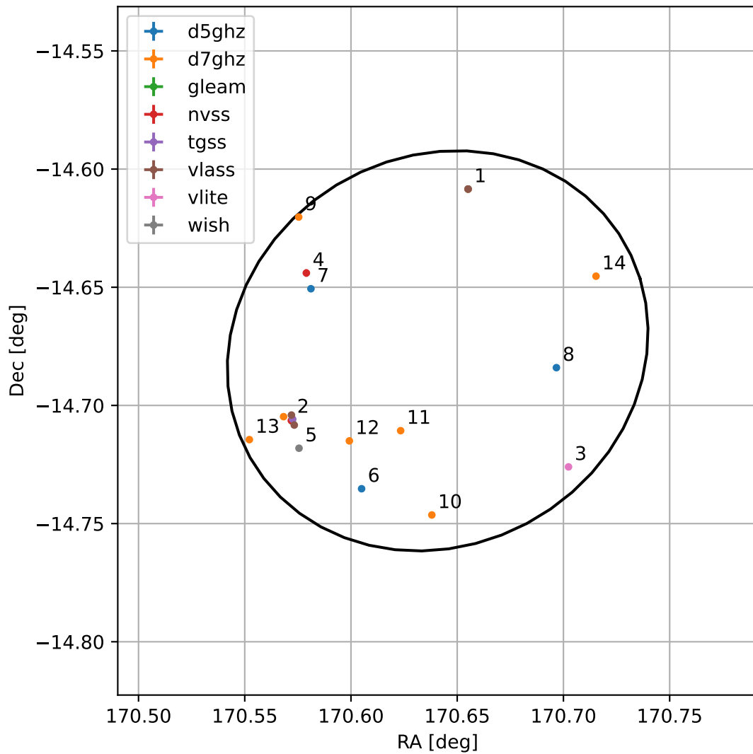
4FGL J1122.5-1440
