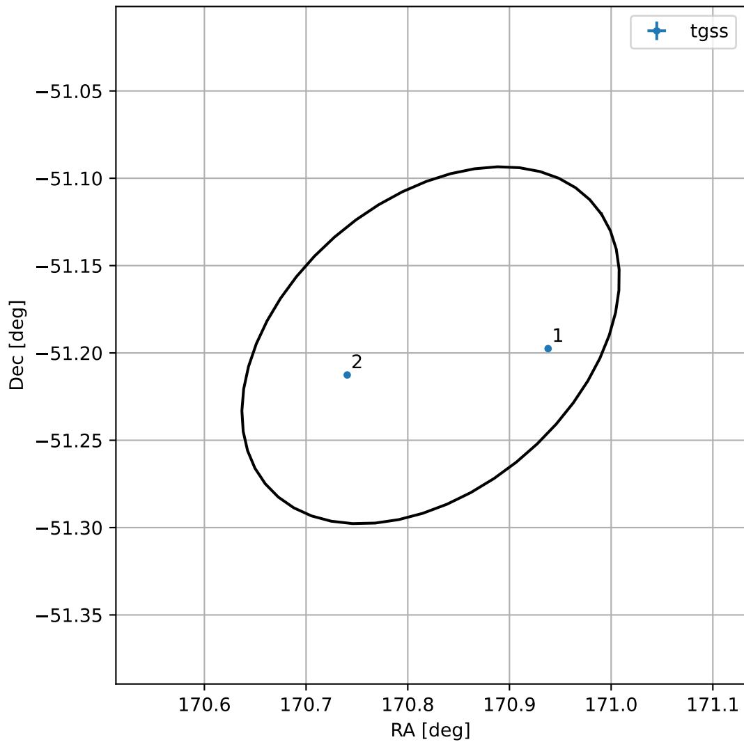
4FGL J1123.2-5111
